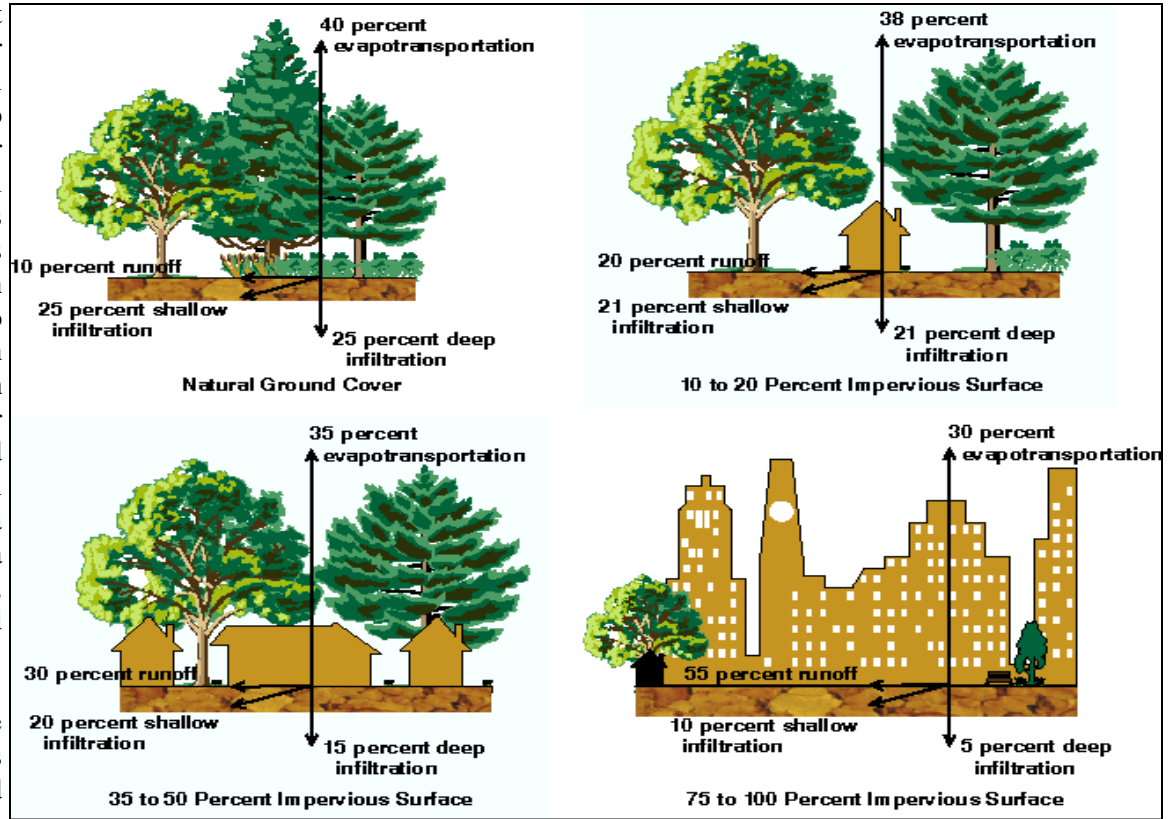
Figure Credit: USGS
